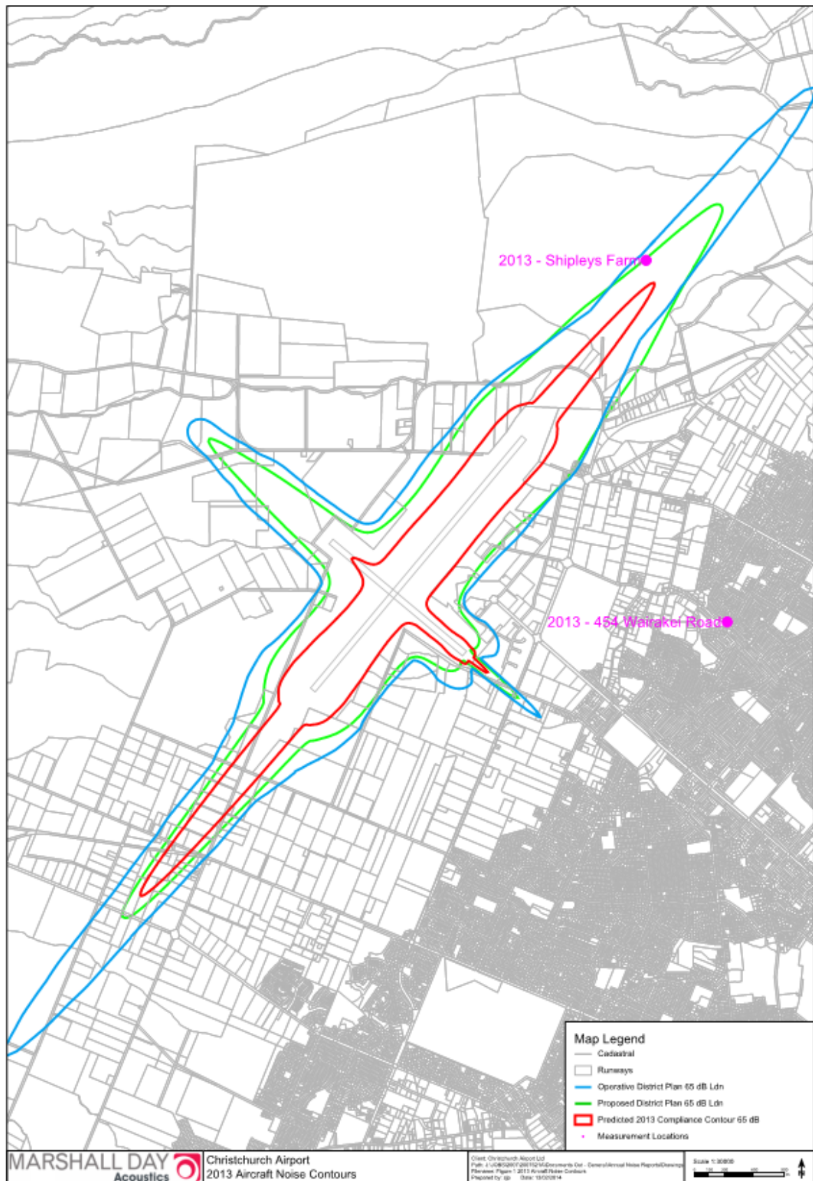
Figure 1: Noise from Aircraft Operations 2013 Compared with City Plan Limit
