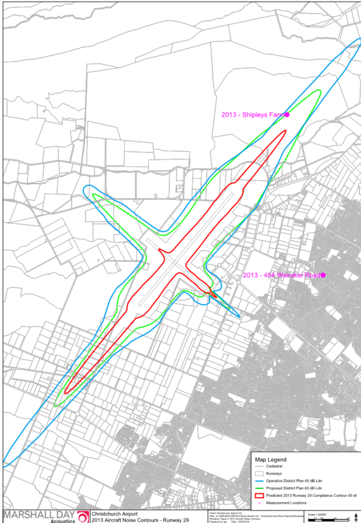
Figure 2: Noise from Aircraft Operations 2013 Runway 29 use Compared with City Plan Limit
